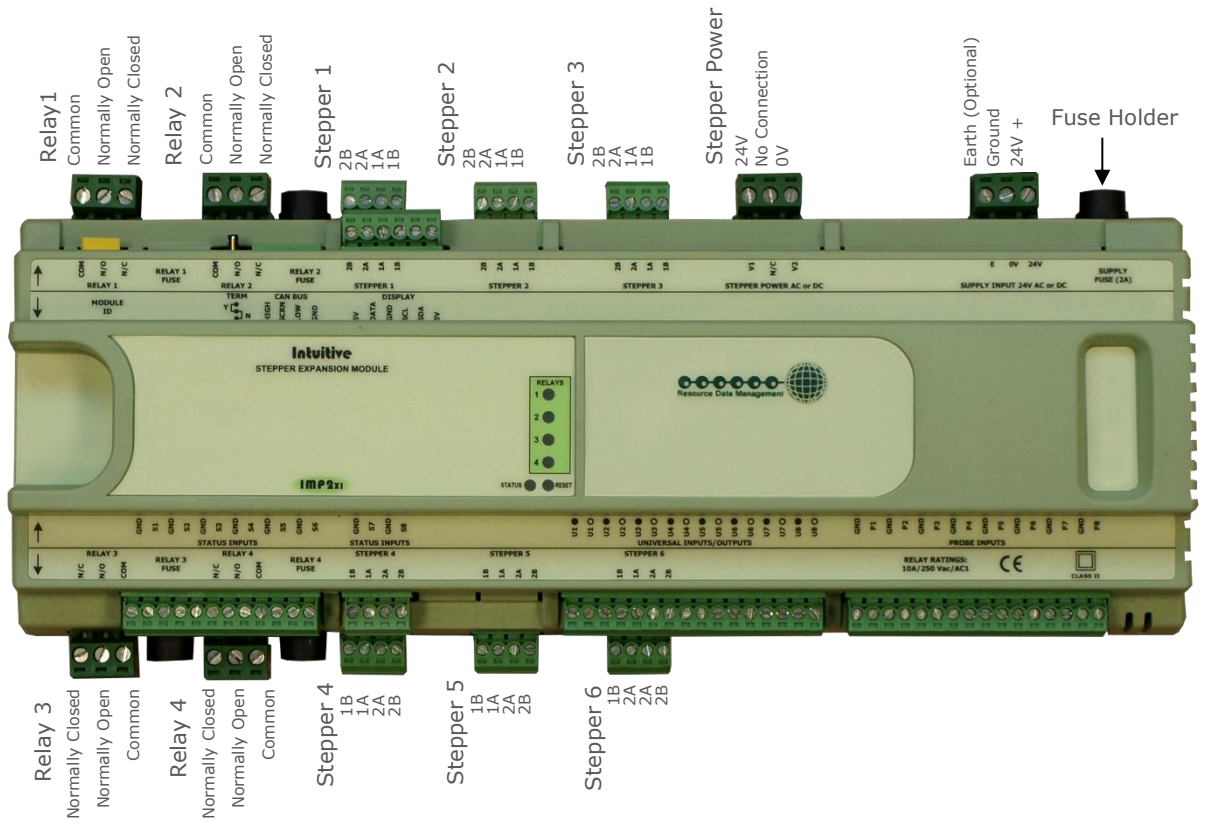
PR0660 Bottom Row Connections
