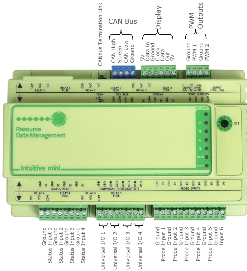
PR0681 Top Row Connections
