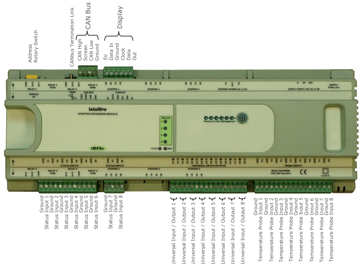
PR0660 Top Row Connections
