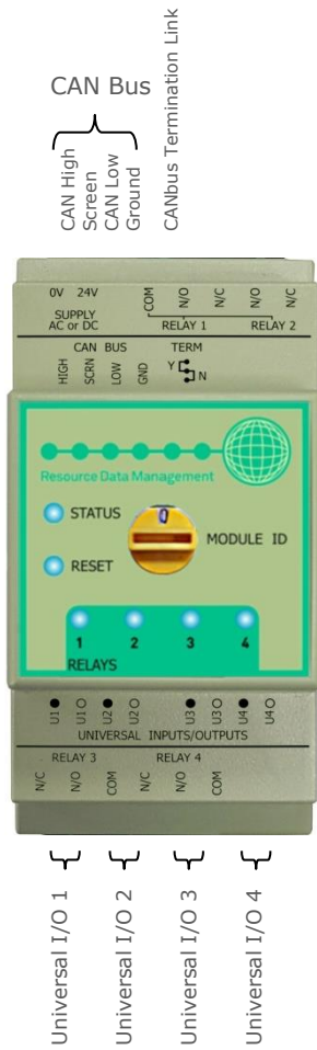
PR0663 4-4 Top Row Connections
