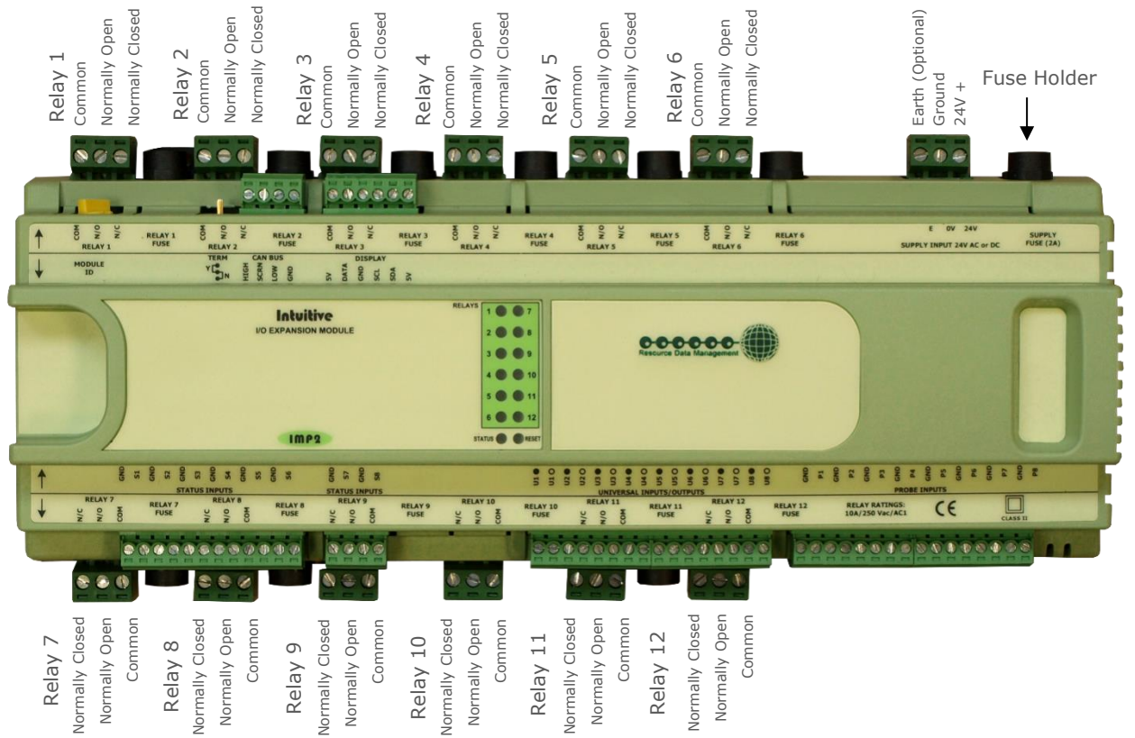
PR0661 Bottom Row Connections
