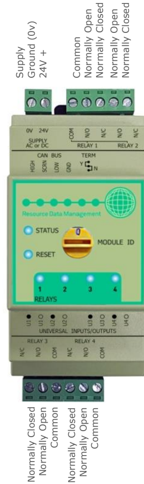
PR0663 4-4 Bottom Row Connections
