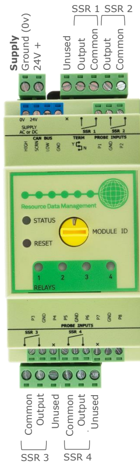
PR0663 8P-4E Top Row Connections
